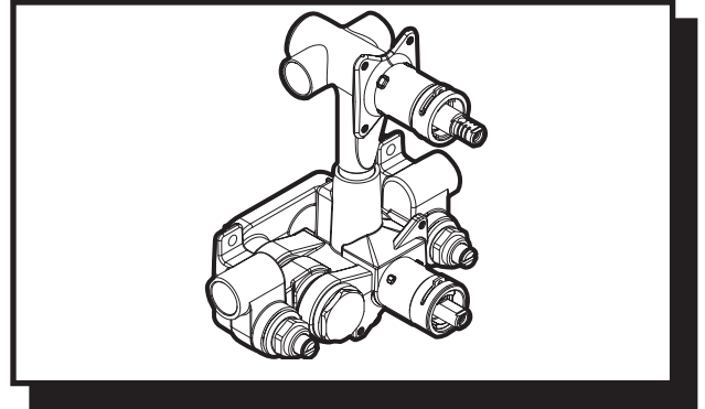
MOENTROL® 3-Function Built In Transfer Valve
